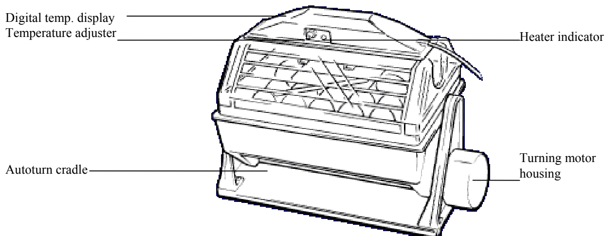
Fig. 1 Functional features of the Octagon 20 and Autoturn cradle (Octagon 40 functionally similar).
