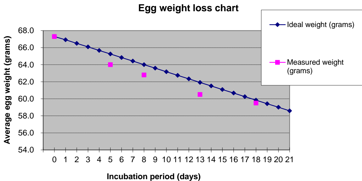
The graph above shows the average actual weights of incubating eggs against the ideal weight loss line - Note that the greater than ideal weight loss in the earlier stages of incubation has been corrected by hatching day.
